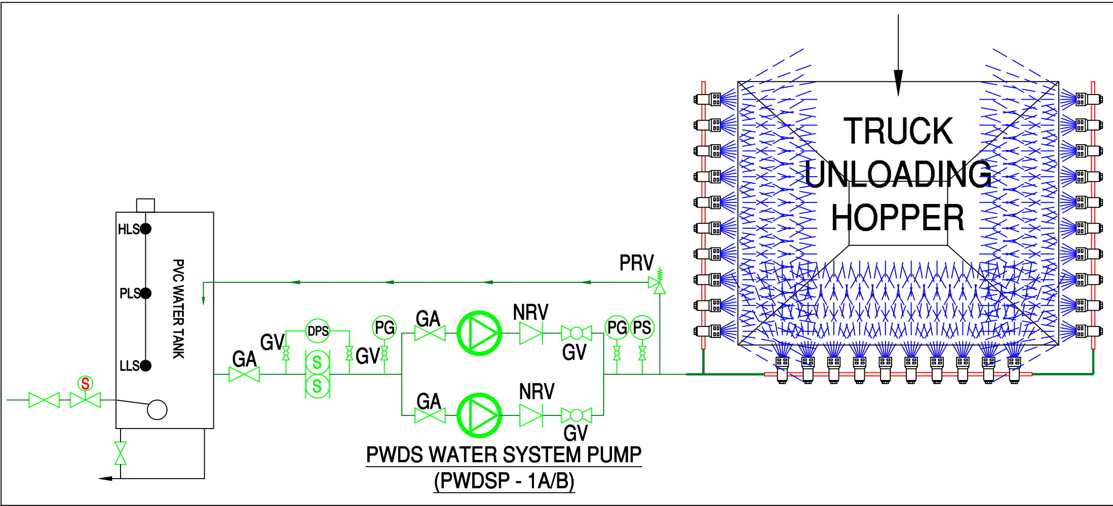
PLAIN WATER DUST SUPPRESSION SYSTEM FOR TRUCK UNLOADING HOPPER
